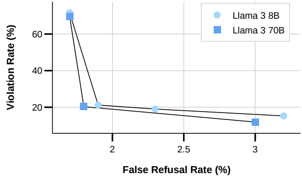
Figure 18 Influence of model size on safety mix design for balancing violation rate (VR) and false refusal rate (FRR). Each point of the scatterplot represents a different data mix balancing safety and helpfulness data. Different model sizes retain varying capacities for safety learning. Our experiments show that 8B models require a higher proportion of safety data relative to helpfulness data in the overall SFT mix to achieve comparable safety performance to 70B models. Larger models are more capable of discerning between adversarial and borderline context, resulting in a more favorable balance between VR and FRR.
