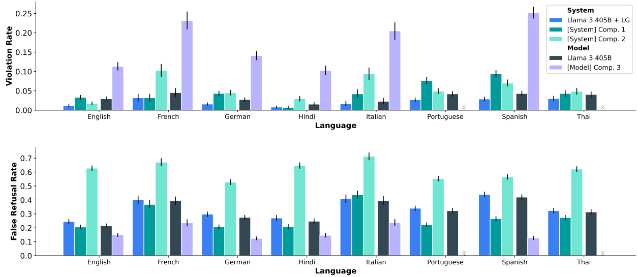
Figure 19 Violation rates (VR) and false refusal rates (FRR) on English and our core multilingual short context benchmarks, comparing Llama 3 405B—with and without Llama Guard (LG) system-level protections—to competitor models and systems. Languages not supported by Comp. 3 represented with an ‘x.’ Lower is better.
